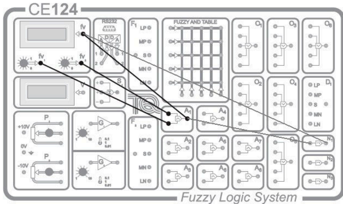
Figure 7: Fuzzy Logic Operator
