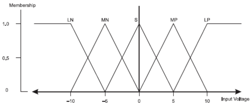
Figure 2: Fuzzy Membership Functions for a Five Level Fuzzifier
