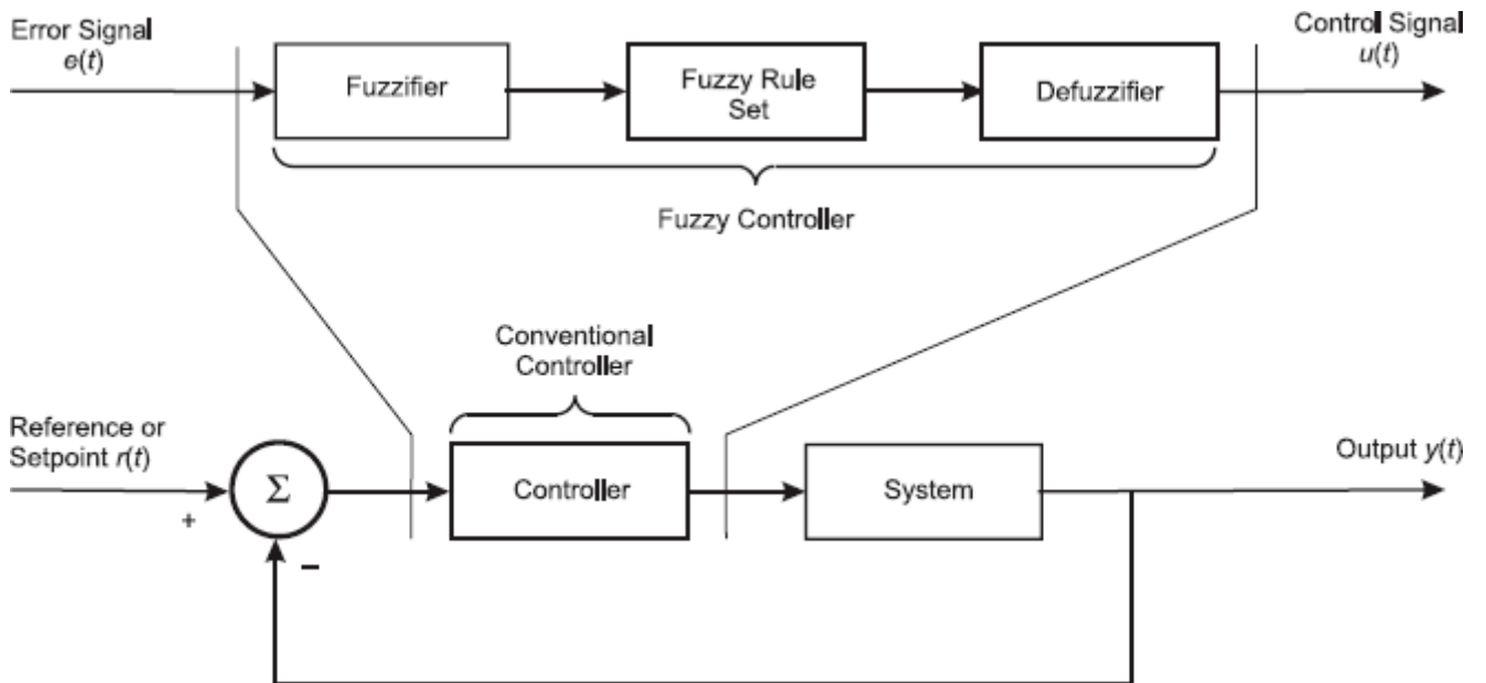
Figure 1: Fuzzy Controller
