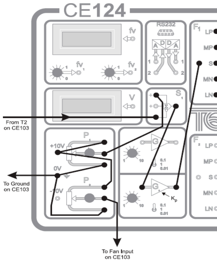
Figure 8: Fuzzy Control Wiring Diagram 1
